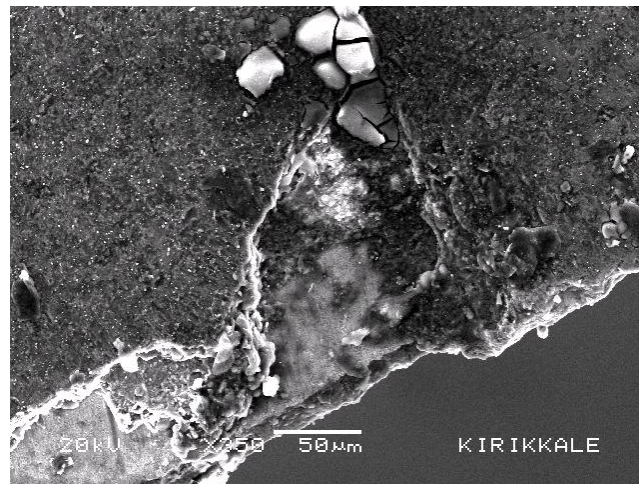
Figure 3. SEM image of the worn uncoated cemented carbide tool used for machining Al-SiC 16%-30 µm MMC at 20 m/min showing three-body abrasion
