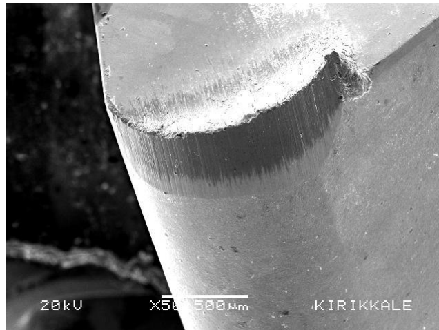
Figure 4. SEM image of the worn diamond coated cemented carbide tool used for machining Al-SiC 8%-30 µm MMC at 25 m/min.
